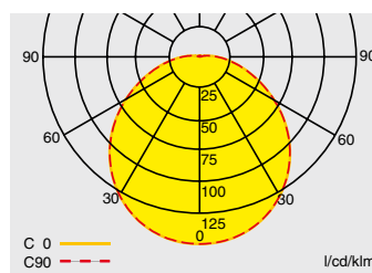
Light distribution curve 84022 CG-S
