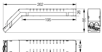
Module housing
