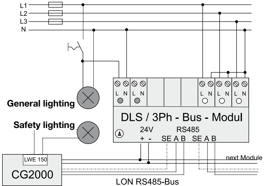
fig. 3: Wiring of the DLS/3PH BUS-Module
