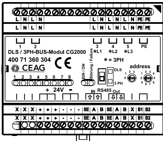
fig 1 Connections DLS/3PH Modul
